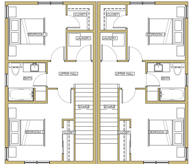
Second Floor
