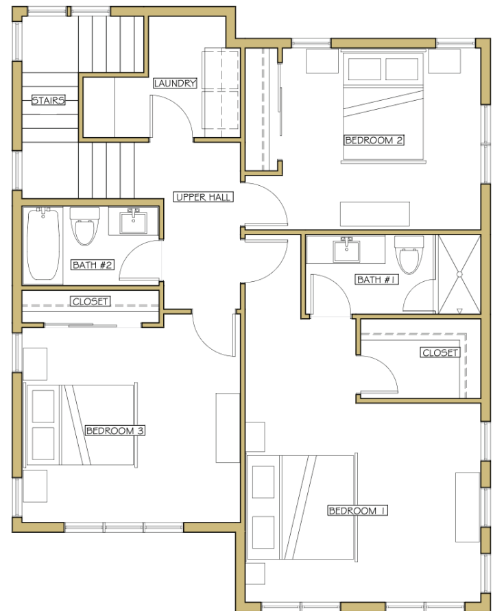
Second Floor
